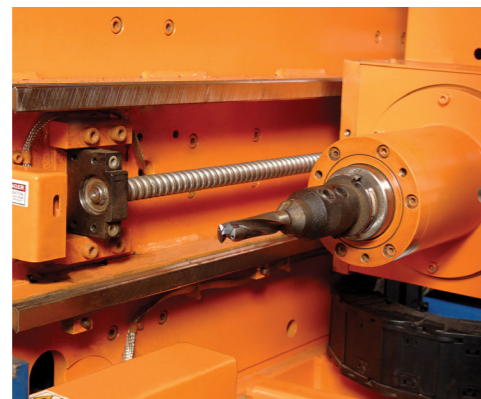
■ PRECISION BALL SCREW SPINDLE FEED
