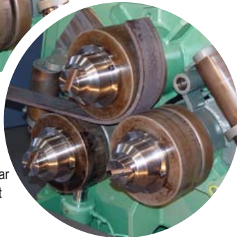
Flat bar on-edge
